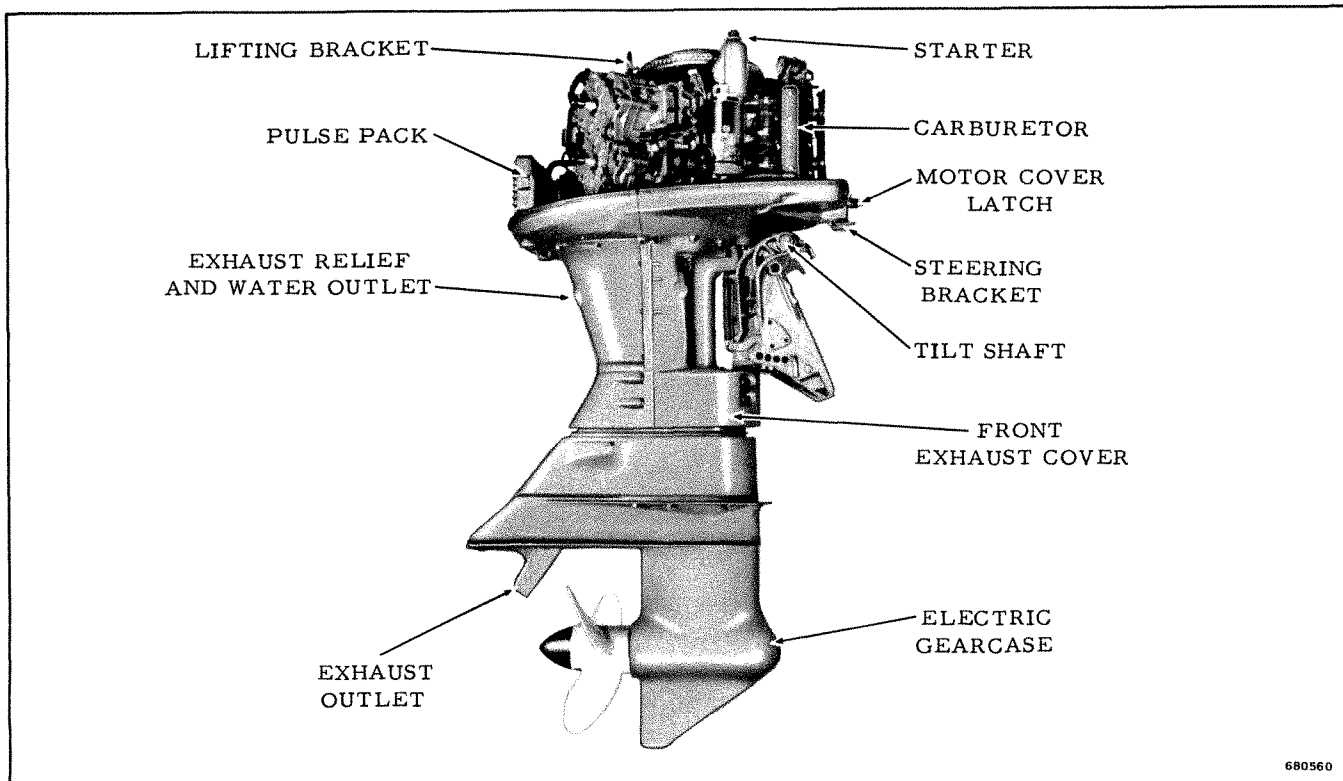
Figure 1-1. Starboard Side
