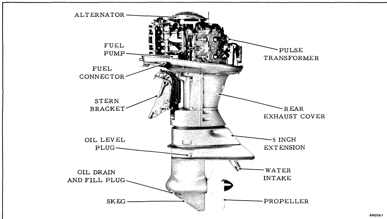
Figure 1-1. Starboard Side
